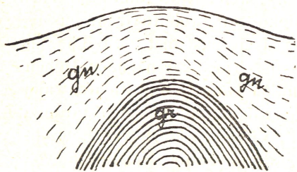
gr. Granit. gn. Gneiss.
